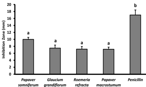
Figure 3. Antimicrobial activity of alkaloids extracts of different plants against S. aureus . Bars represent standard errors. The different letters above the error bars indicate significant differences at the 0.05 level (Student’s t-test: P < 0.05 ).
